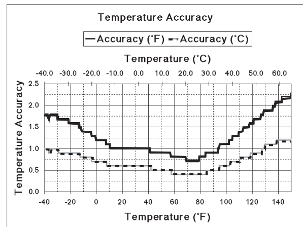
Figure 2: External Temperature Probe Accuracy
